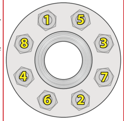
Illustration 57 Lug Nut Torque Sequence... Follow the Sequence Below to Torque the Lug Nuts
